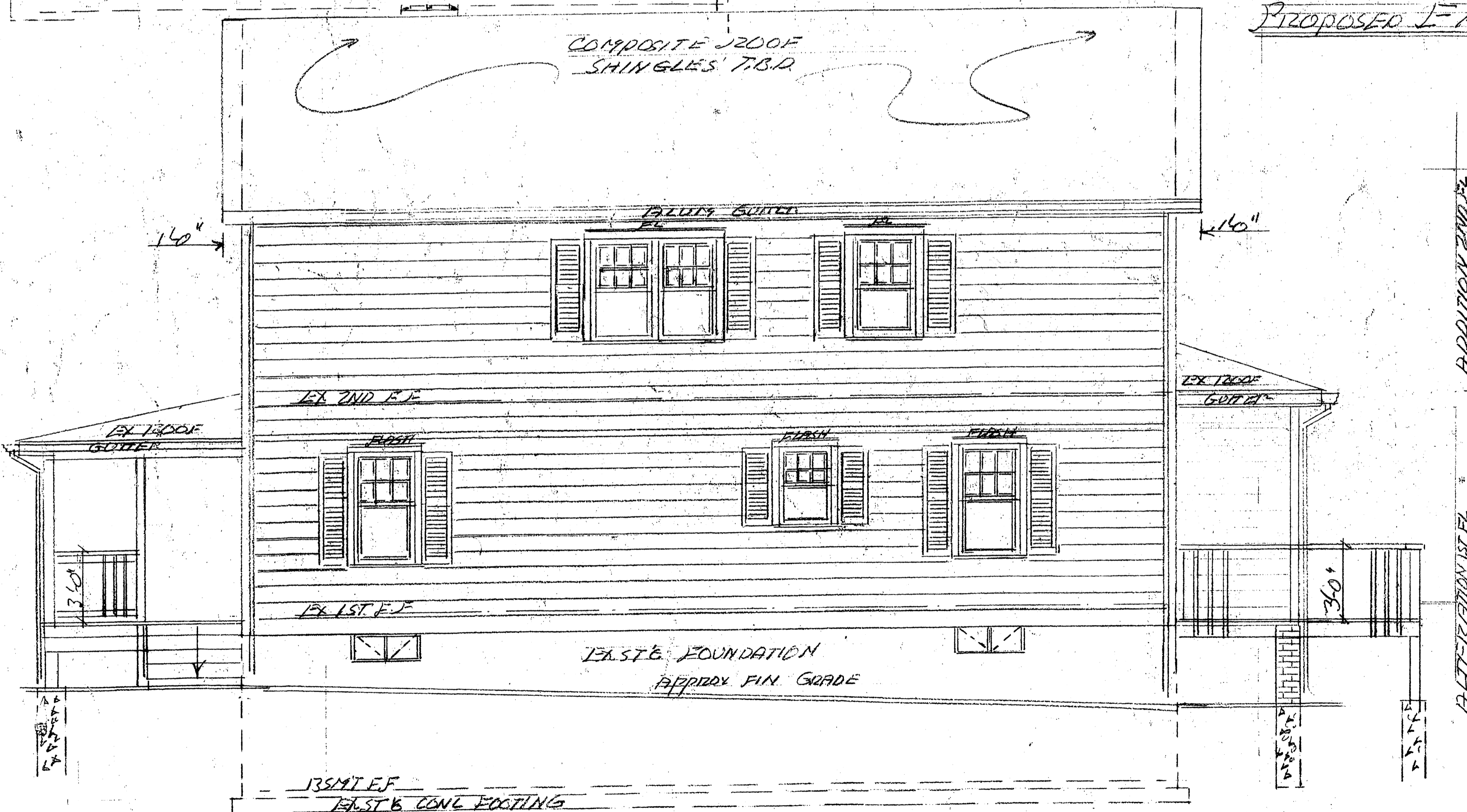
PROPOSED WEST ELEVATION 1/4"=1'-0"
