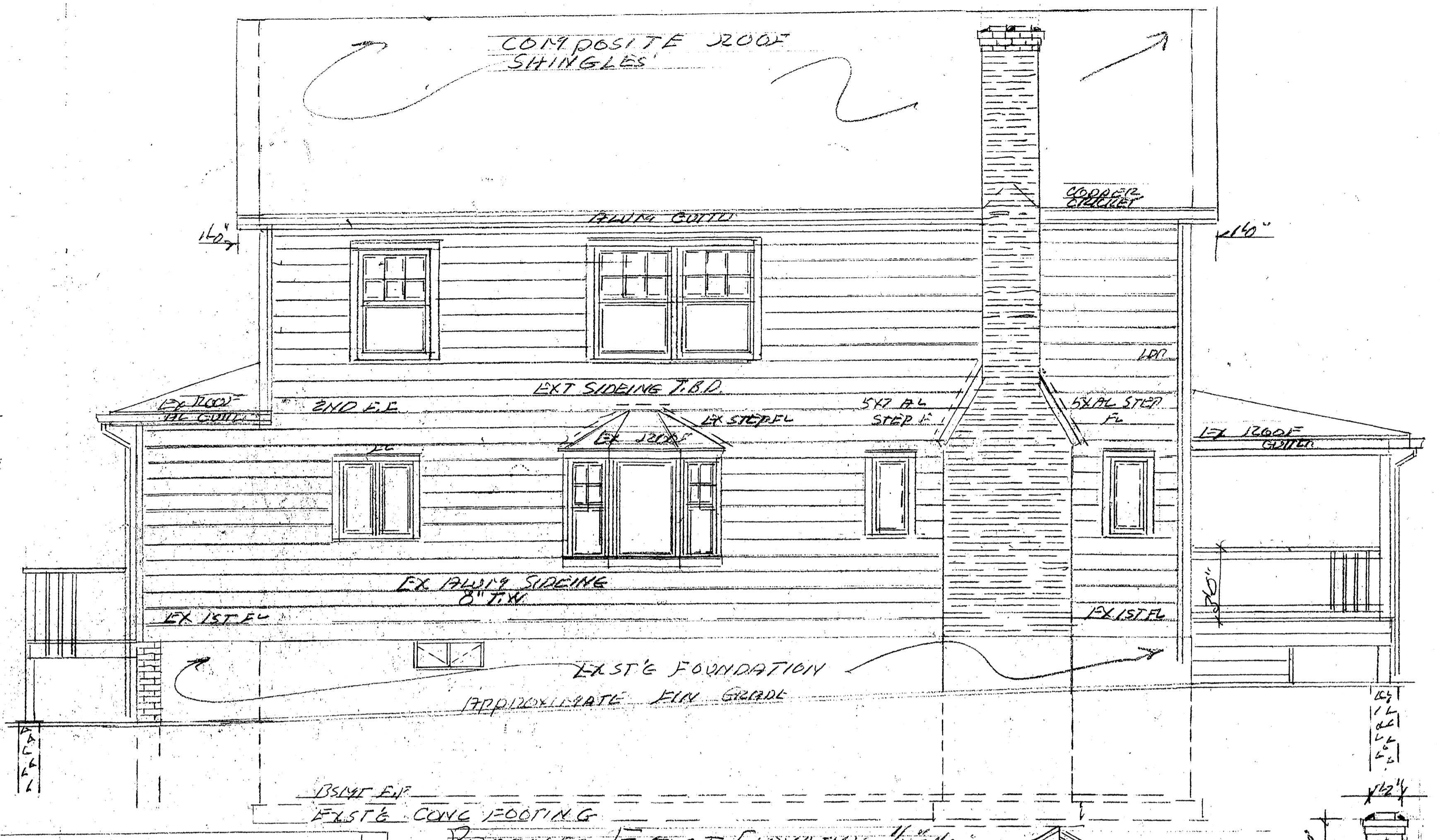
PROPOSED EAST ELEVATION 1/4"=1'-0"
