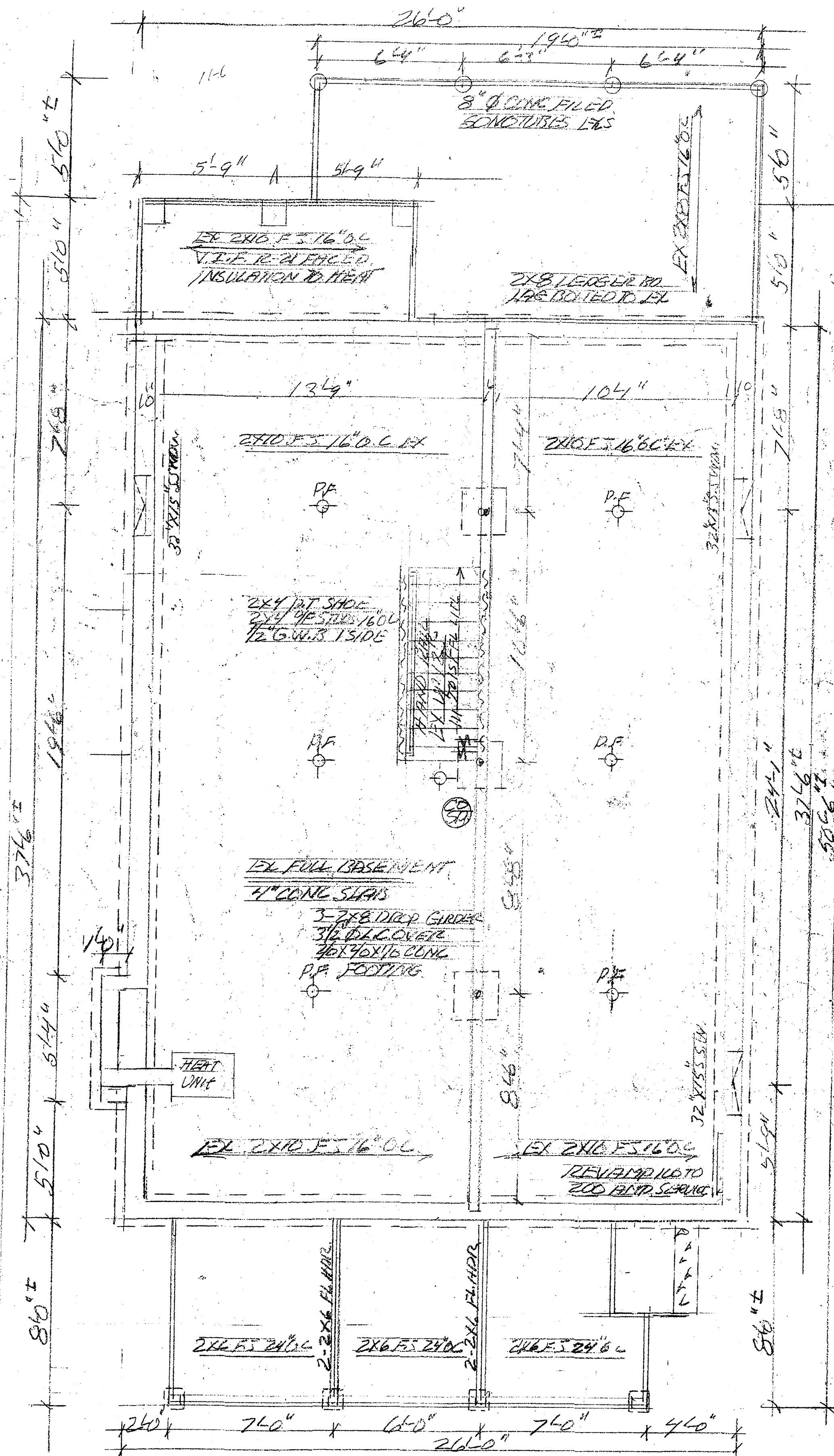
EXIST'G FOUNDATION PLAN 1/2"
